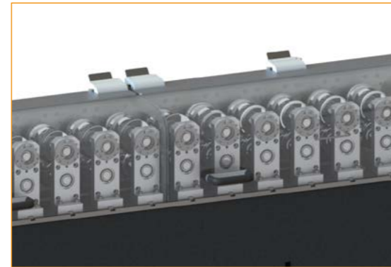
Set of rolling wheels including heat treatment (hardening)
