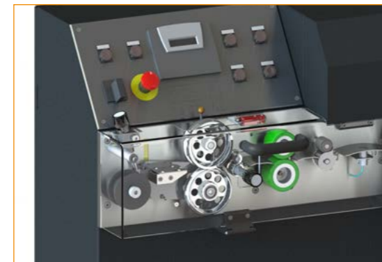
Forming section
